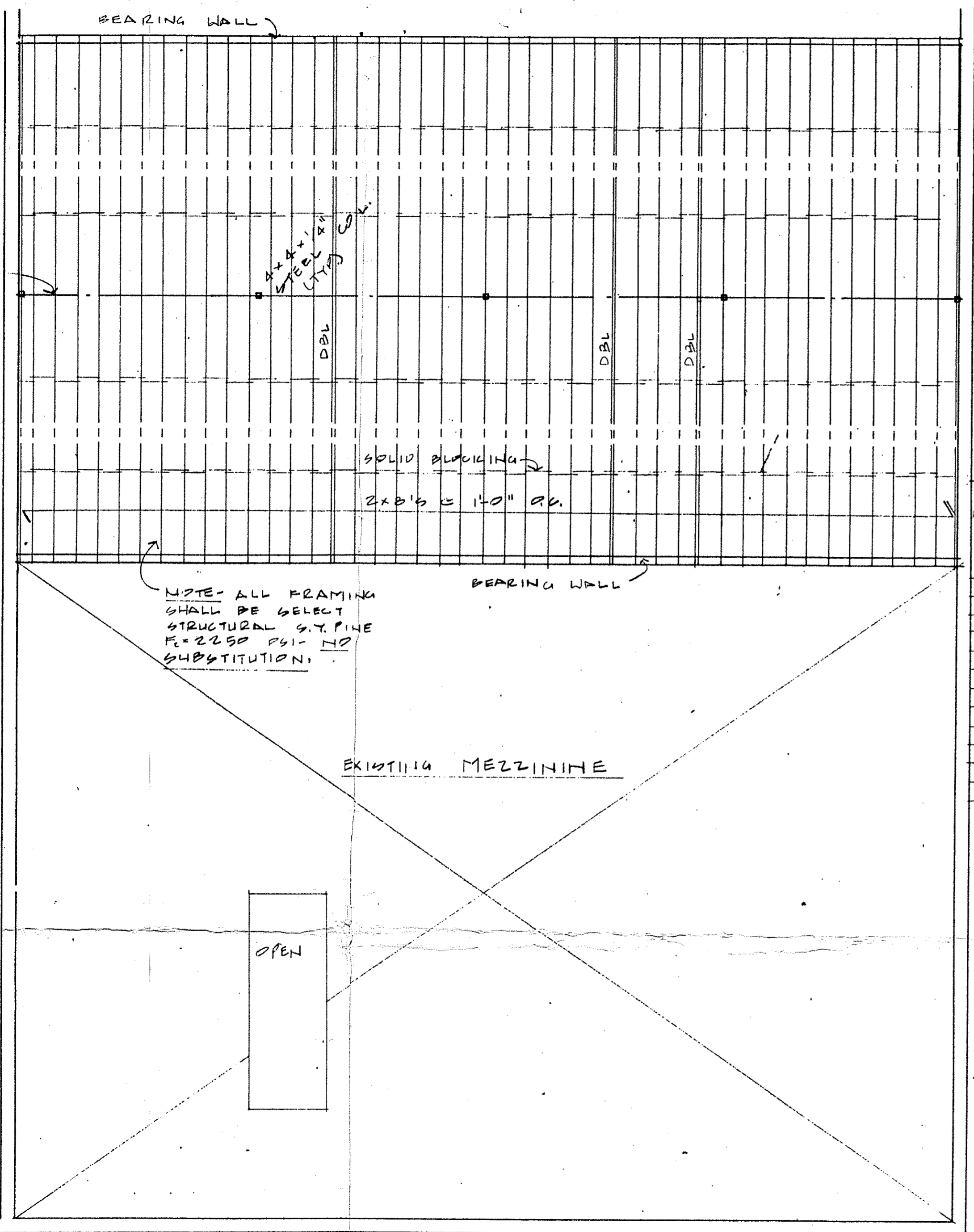
MEZZANINE FRAMING PLAN 1/4"
