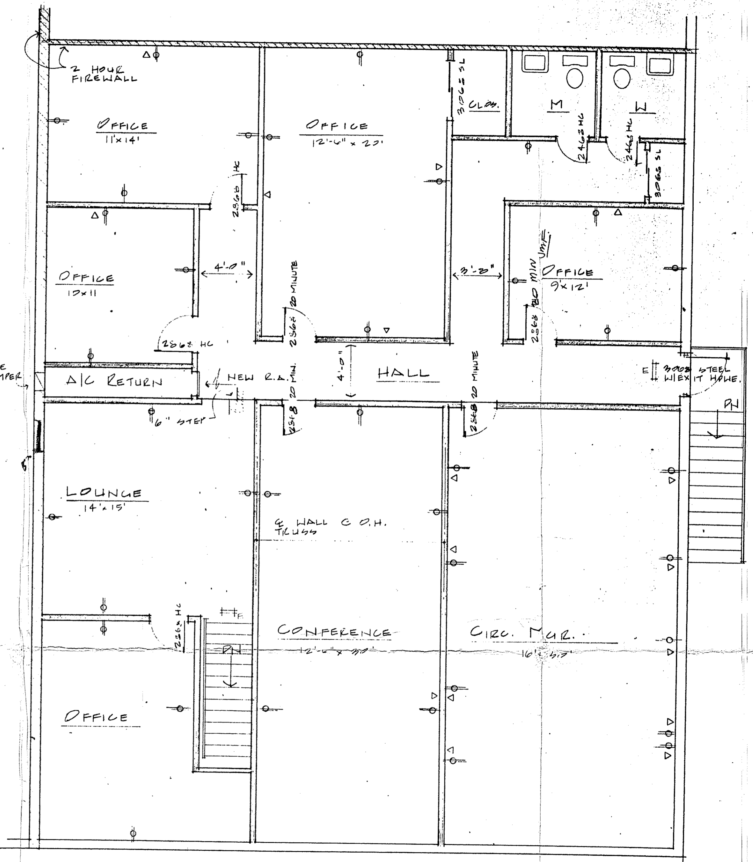
MEZZANINE PLAN 1/4"
